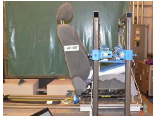
Photo 1. Seat mounted in test fixture. Test platform angle is adjustable relative to seat form. Seat was pulled rearward during test.
