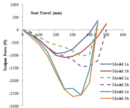
Figure 1. Comparison of tests of three model seats.
