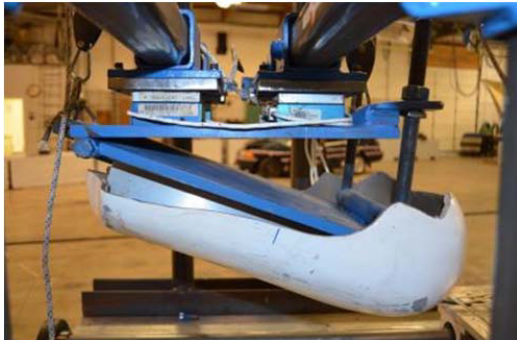
Photo 2. Fiberglass seat form mounted to instrumented platform.
